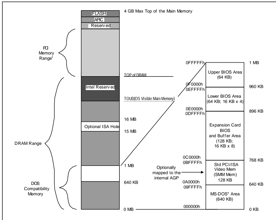
Figure 7. Detailed Memory System Address Map
