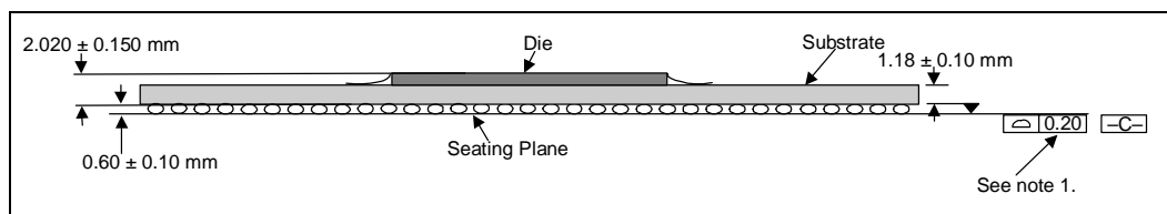
Figure 15. Intel® E7210 MCH Package Dimensions (Side View)
