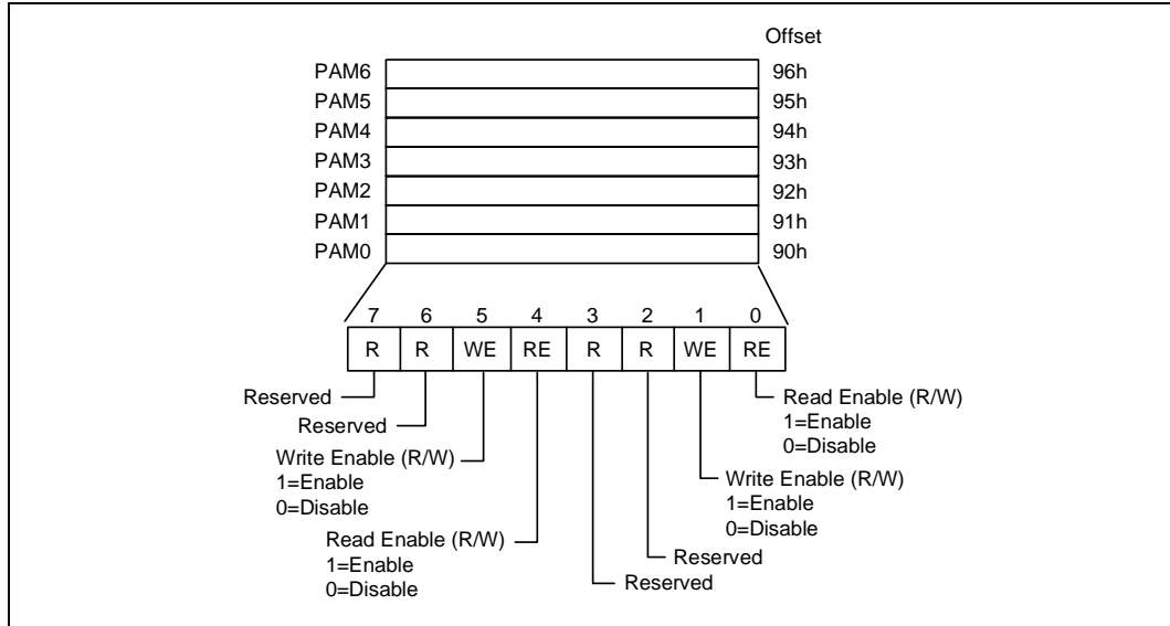
Figure 6. PAM Register Attributes
