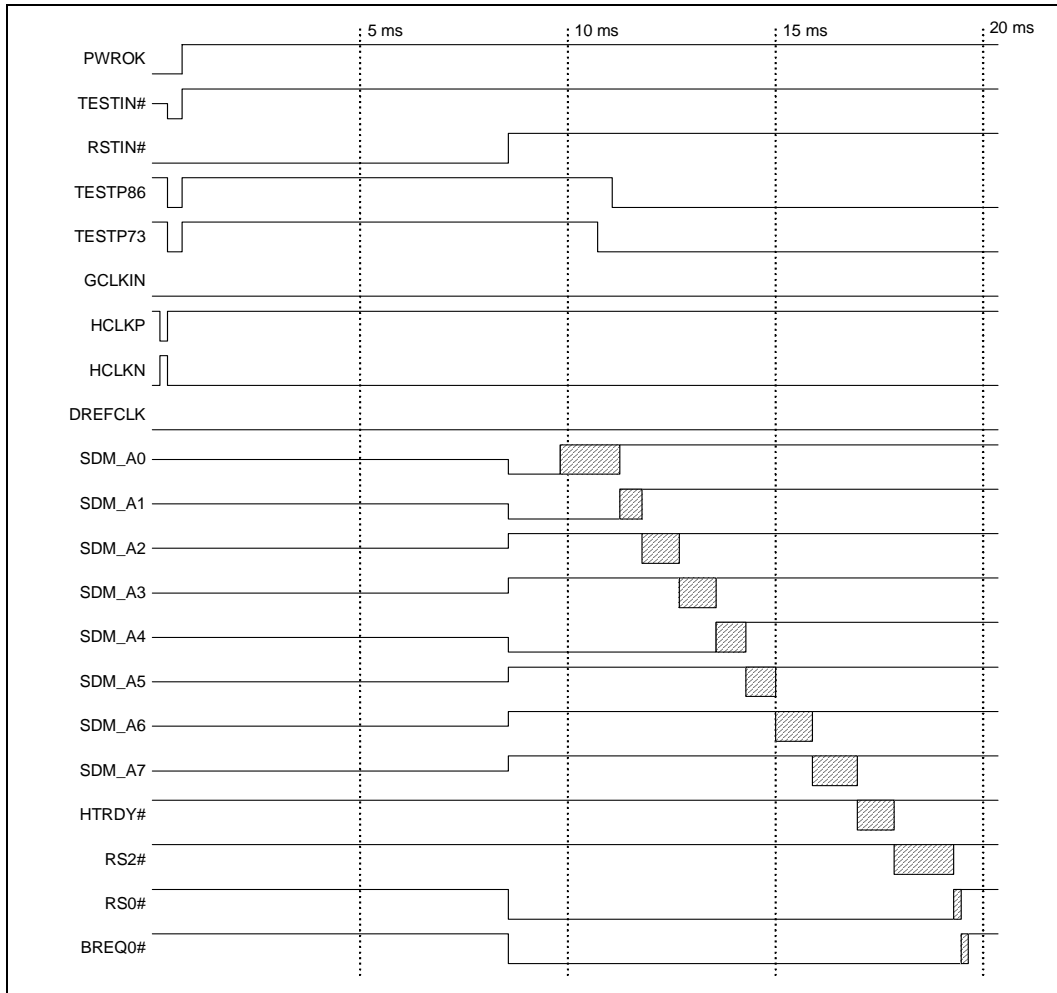
Figure 18. XOR Testing Chains Tested Sequentially
