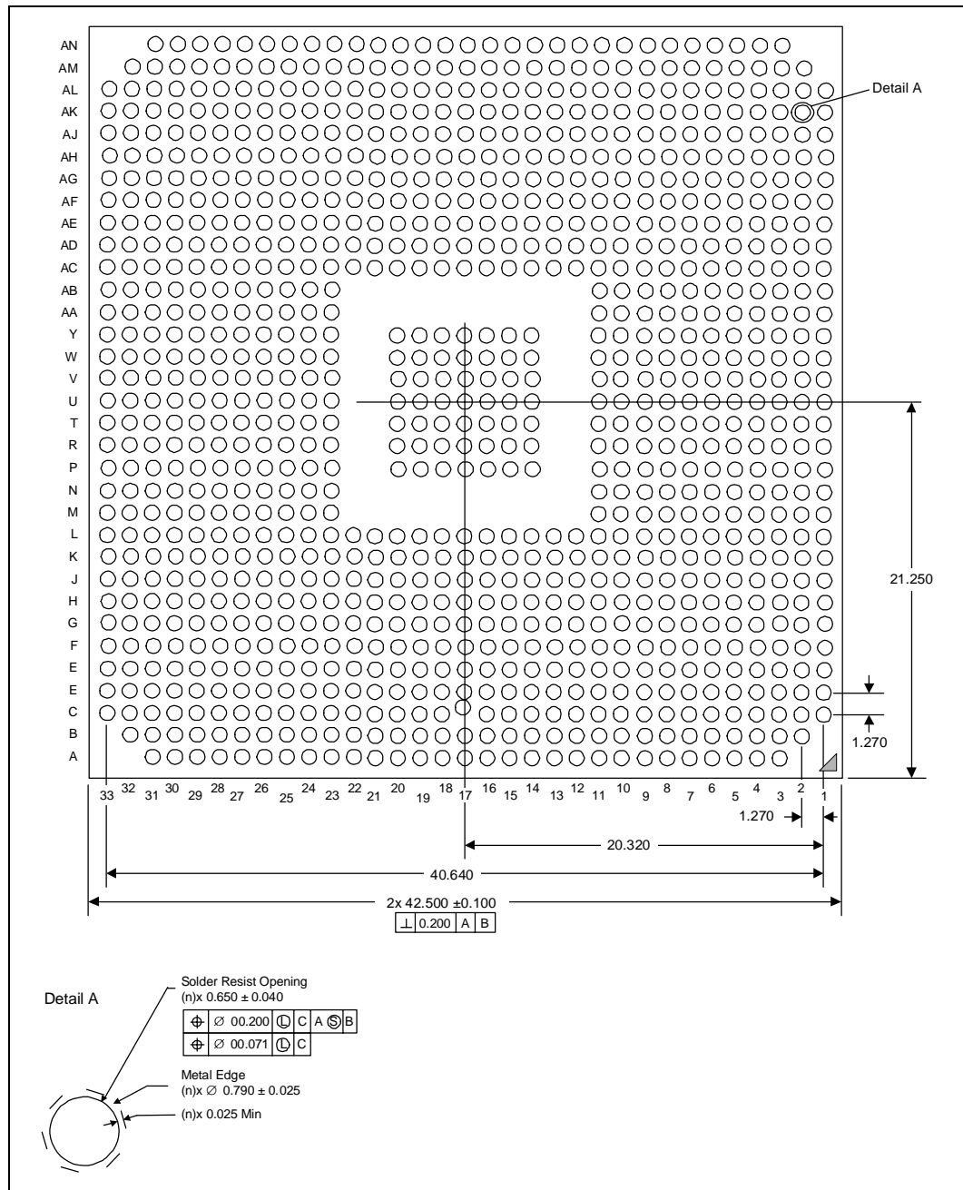
Figure 16. Intel® E7210 MCH Package Dimensions (Bottom View)
